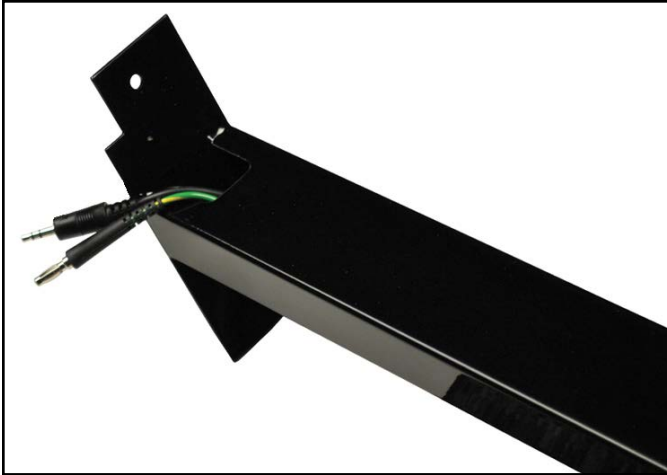
Figure 6. Routing the ground and foot plate cords through the pedestal
